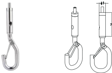
Cable Looper HK-0041
