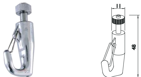
HK-0006B (1.5mm cable only)
